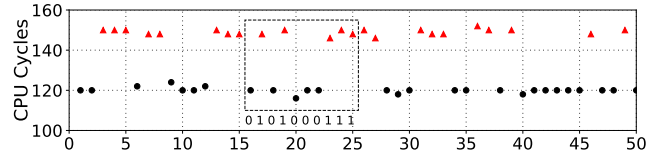
Fig. 10: Latency traces for a 50-bit transmission by Spy corresponding to the covert channel in Figure 9. Decoding for bit 16-25 is highlighted in the boxes.
