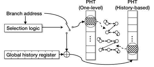
Fig. 1: A high-level illustration of modern branch predictor.
