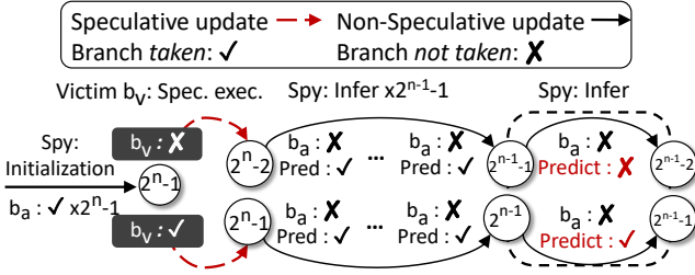
Fig. 8: Possible changes of PHI_t states under exploitation (for n -bit saturating counters). The circled values denote states of the saturating counters at each stage.
